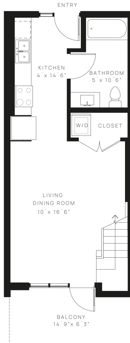
1st Floor
