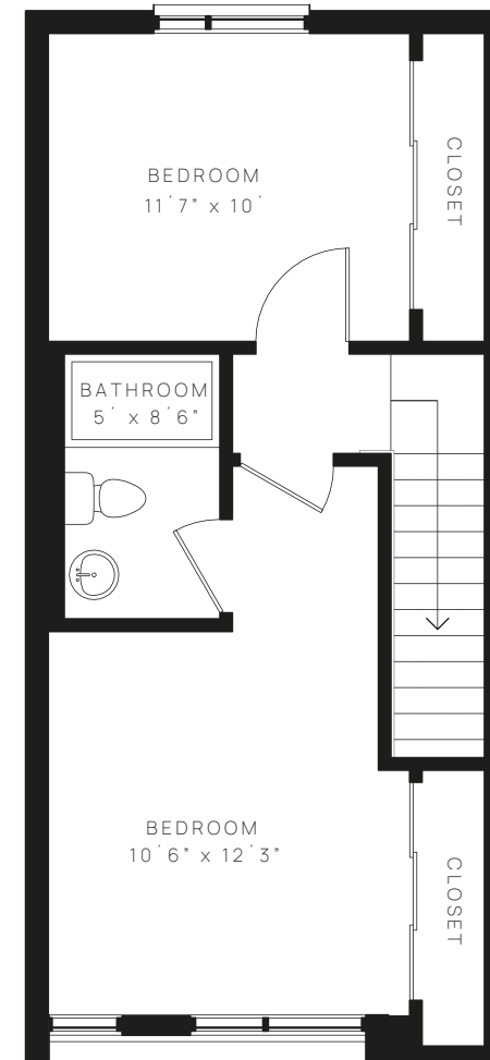
2nd Floor
